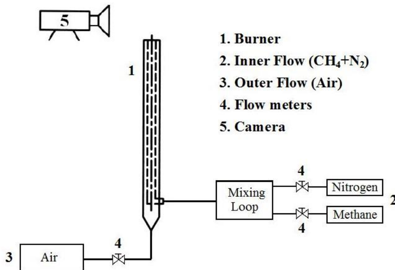
Fig. 1. Schematic of jet flow system.
